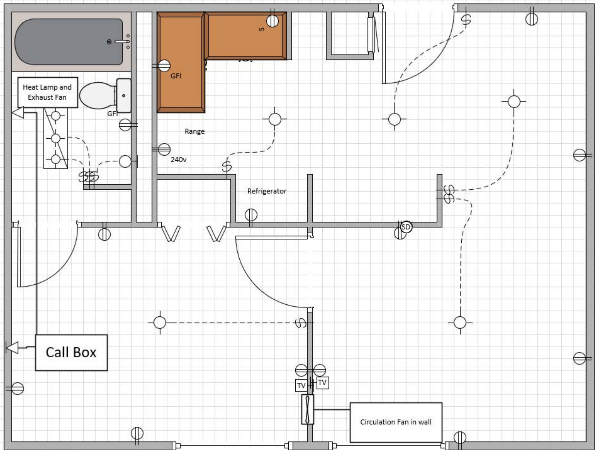
Electrical Layout
